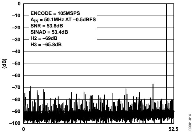
Figure 14. FFT: FS = 105 MSPS, A_{IN} = 50.1 MHz @ -0.5 dBFS, Differential, 1 V p-p Input Range
