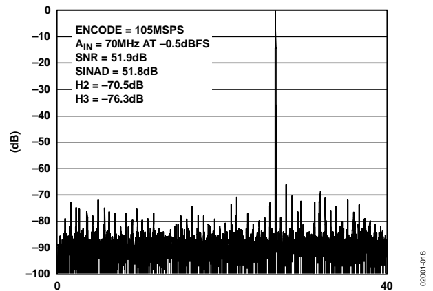
Figure 18. FFT: FS = 105 MSPS A_{IN} = 70 MHz @ -0.5 dBFS, Differential, 1 V p-p Input Range
