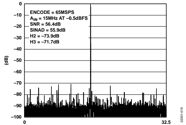
Figure 19. FFT: FS = 65 MSPS, A_{IN} = 15 MHz @ -0.5 dBFS; with AD8138 Driving ADC Inputs, 1 V p-p Input Range
