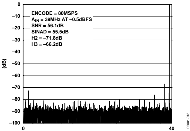
Figure 15. FFT: FS = 80 MSPS, A_{IN} = 39 MHz @ -0.5 dBFS, Differential, 1 V p-p Input Range
