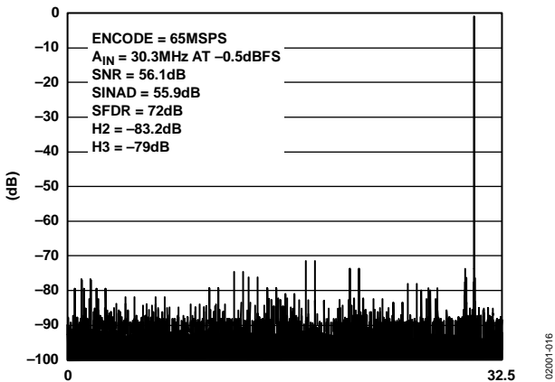
Figure 16. FFT: FS = 65 MSPS, A_{IN} = 30.3 MHz @ -0.5 dBFS, Differential, 2 V p-p Input Range
