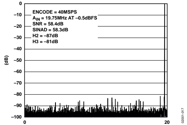
Figure 17. FFT: FS = 40 MSPS, A_{IN} = 19.75 MHz @ -0.5 dBFS, Differential, 1 V p-p Input Range
