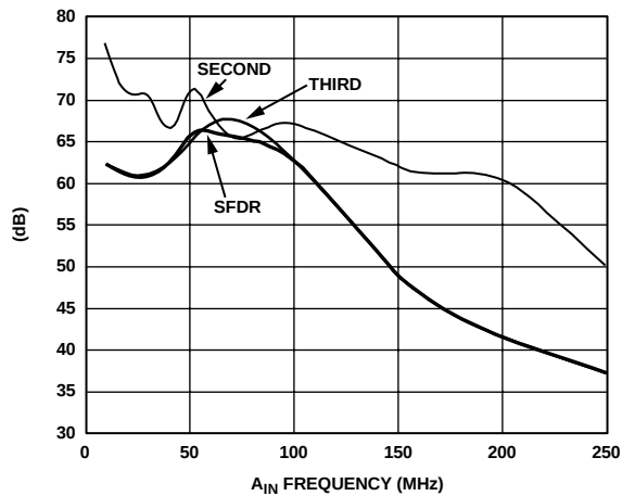
Figure 21. Harmonic Distortion (Second and Third) and SFDR vs. A_{IN} Frequency (1 V p-p, FS = 105\text{ MSPS} )
