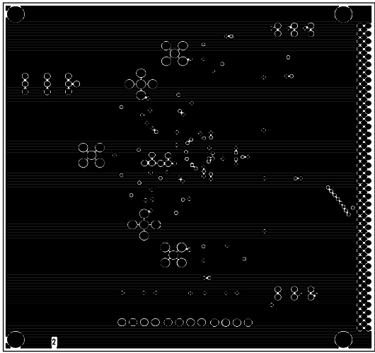
Figure 49. Ground Plane
