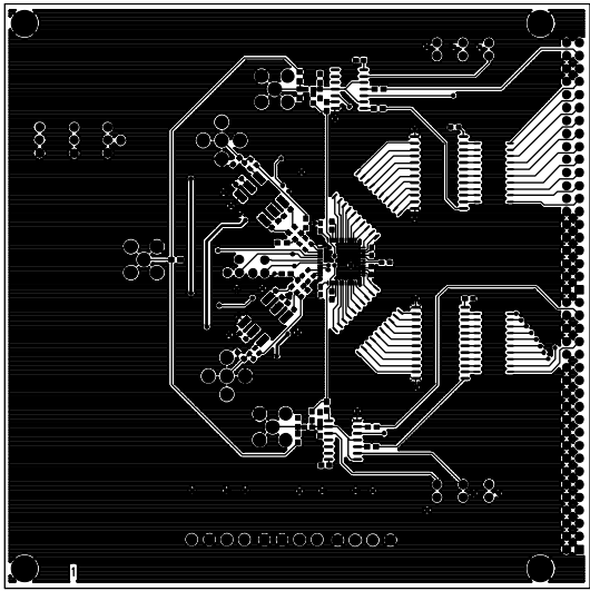
Figure 48. Top Routing
