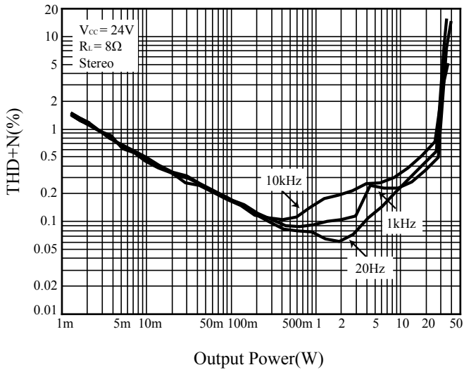
Figure 10 THD+N vs. Output Power
