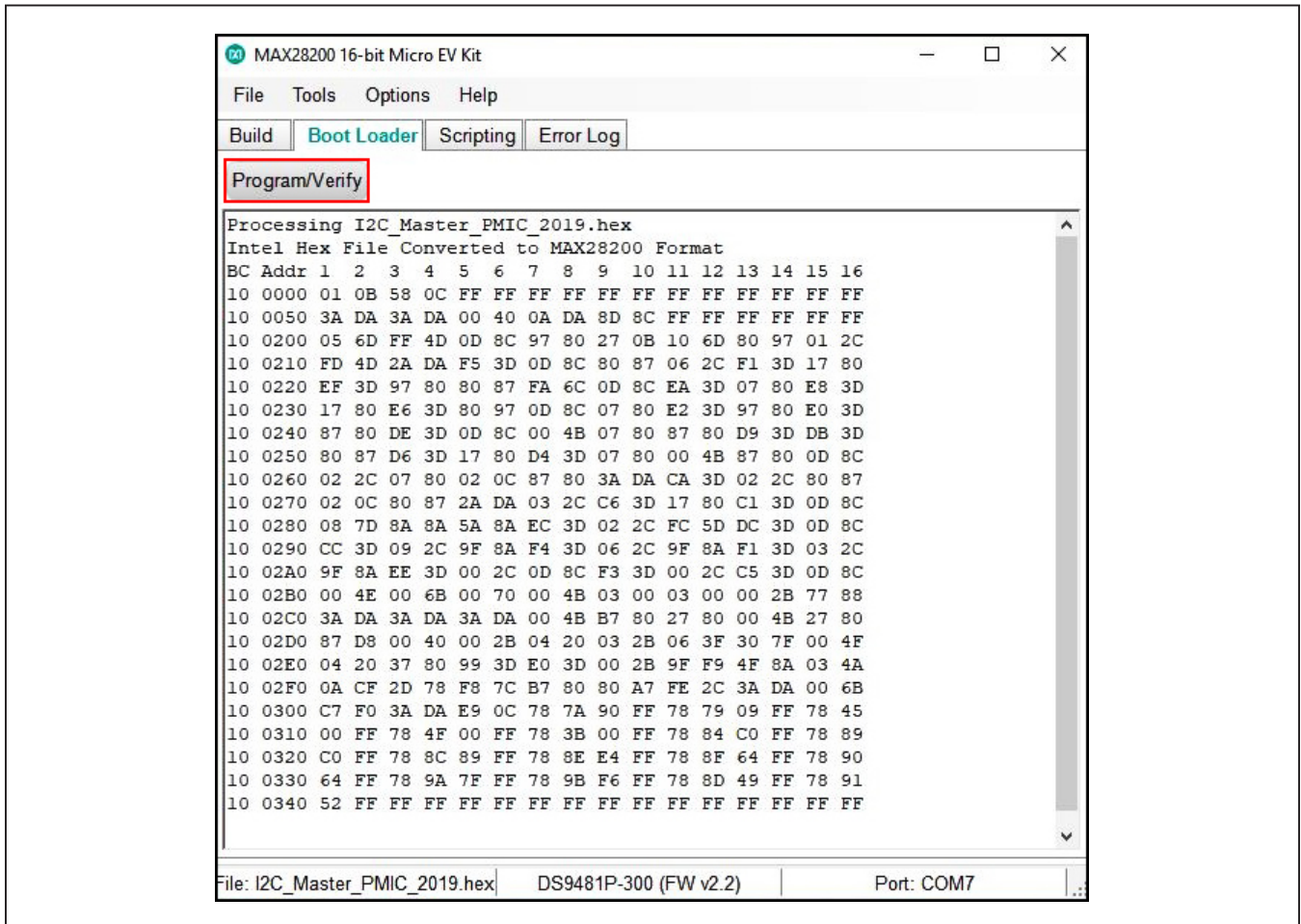
Figure 16. Program the Device with the Data Pattern
