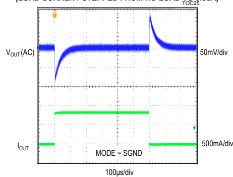
3.3V OUTPUT, PWM MODE, FIGURE 4 CIRCUIT (LOAD CURRENT STEPPED FROM NO LOAD TO 0.85A)
