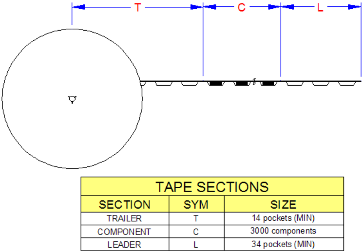
Figure 8.2 36-Pin Package Tape Specifications
