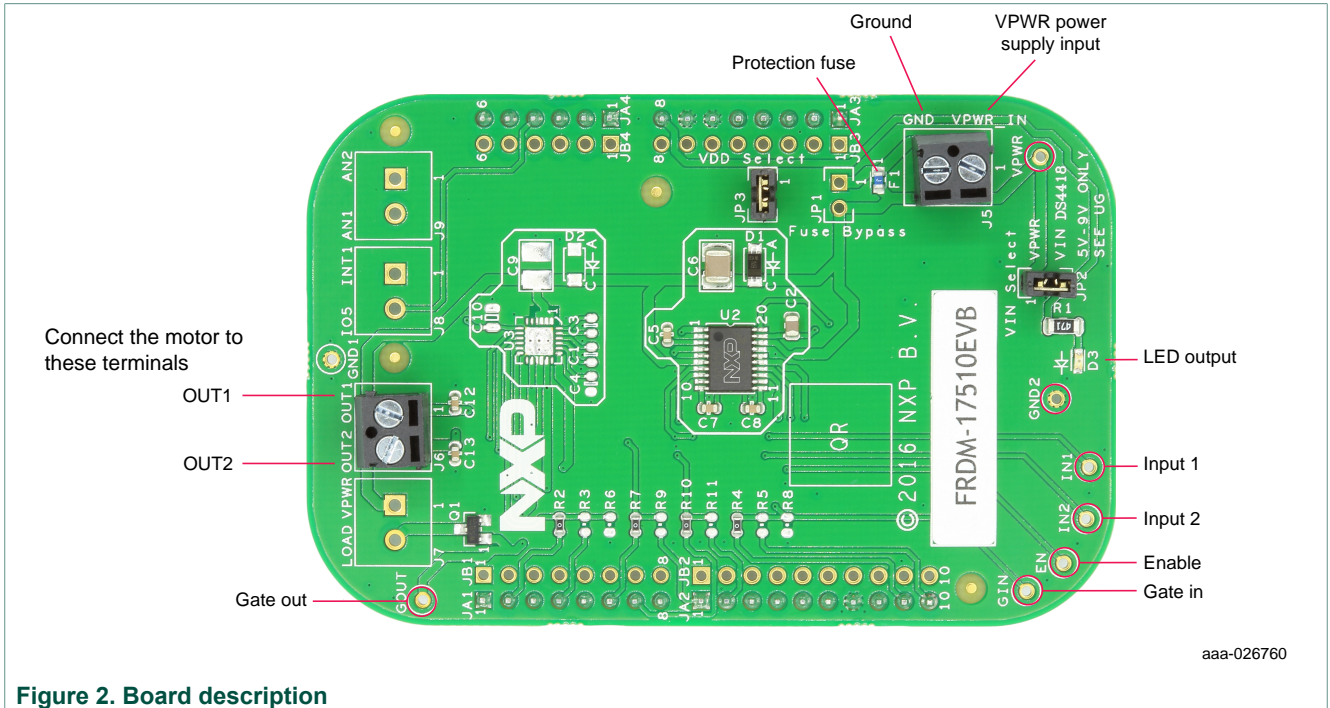
Figure 2. Board description
