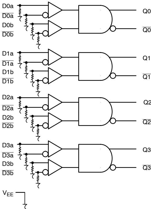
Figure 3. Logic Diagram
