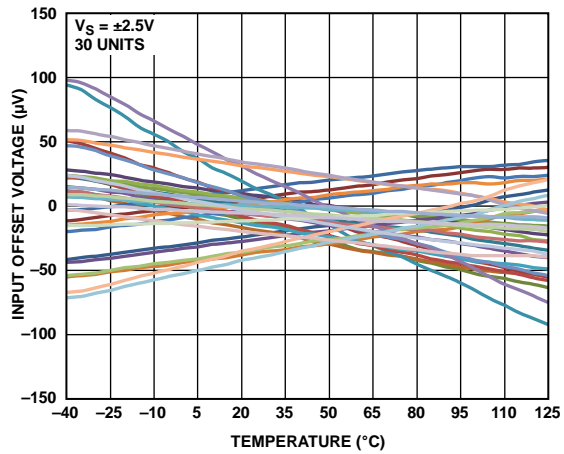
Figure 27. Input Offset Voltage vs. Temperature
