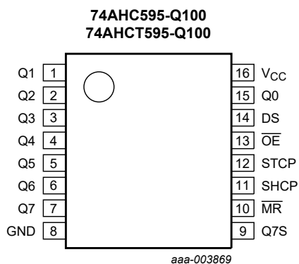
Fig. 5. Pin configuration SOT109-1 (SO16) and SOT403-1 (TSSOP16)
