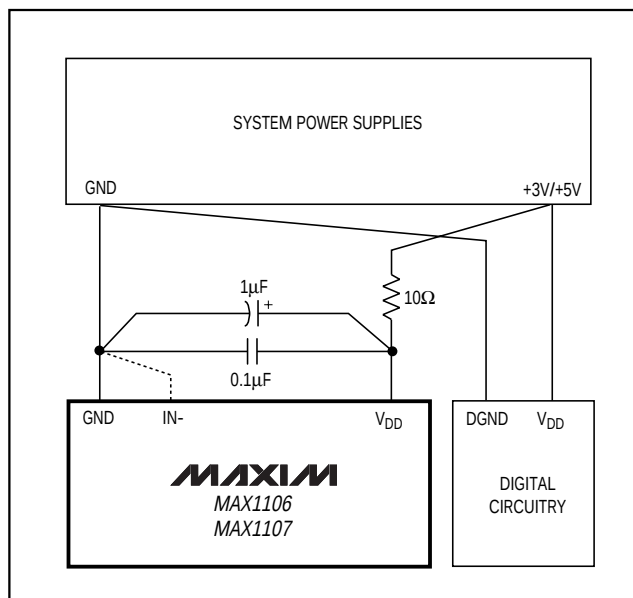
Figure 10. Power-Supply Connections
