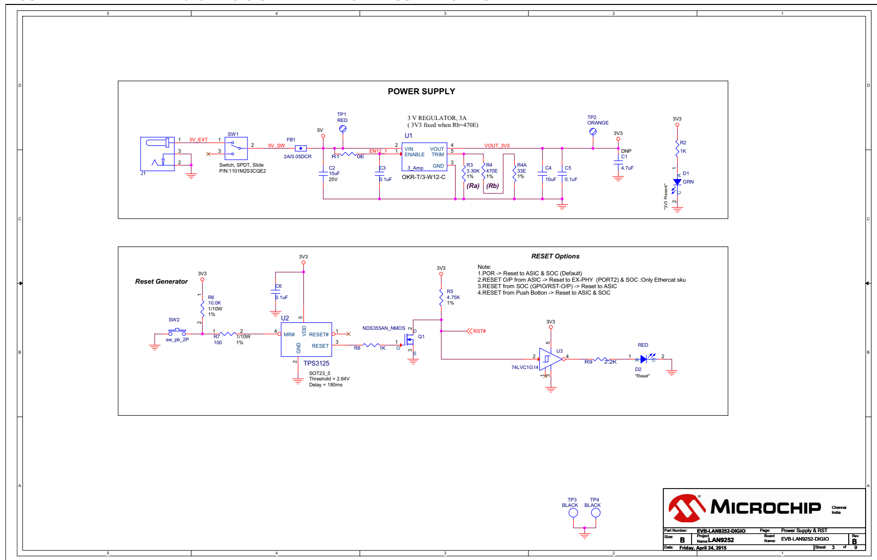
FIGURE B-1: EVB-LAN9252-DIGIO SCHEMATIC POWER SUPPLY & RESET
