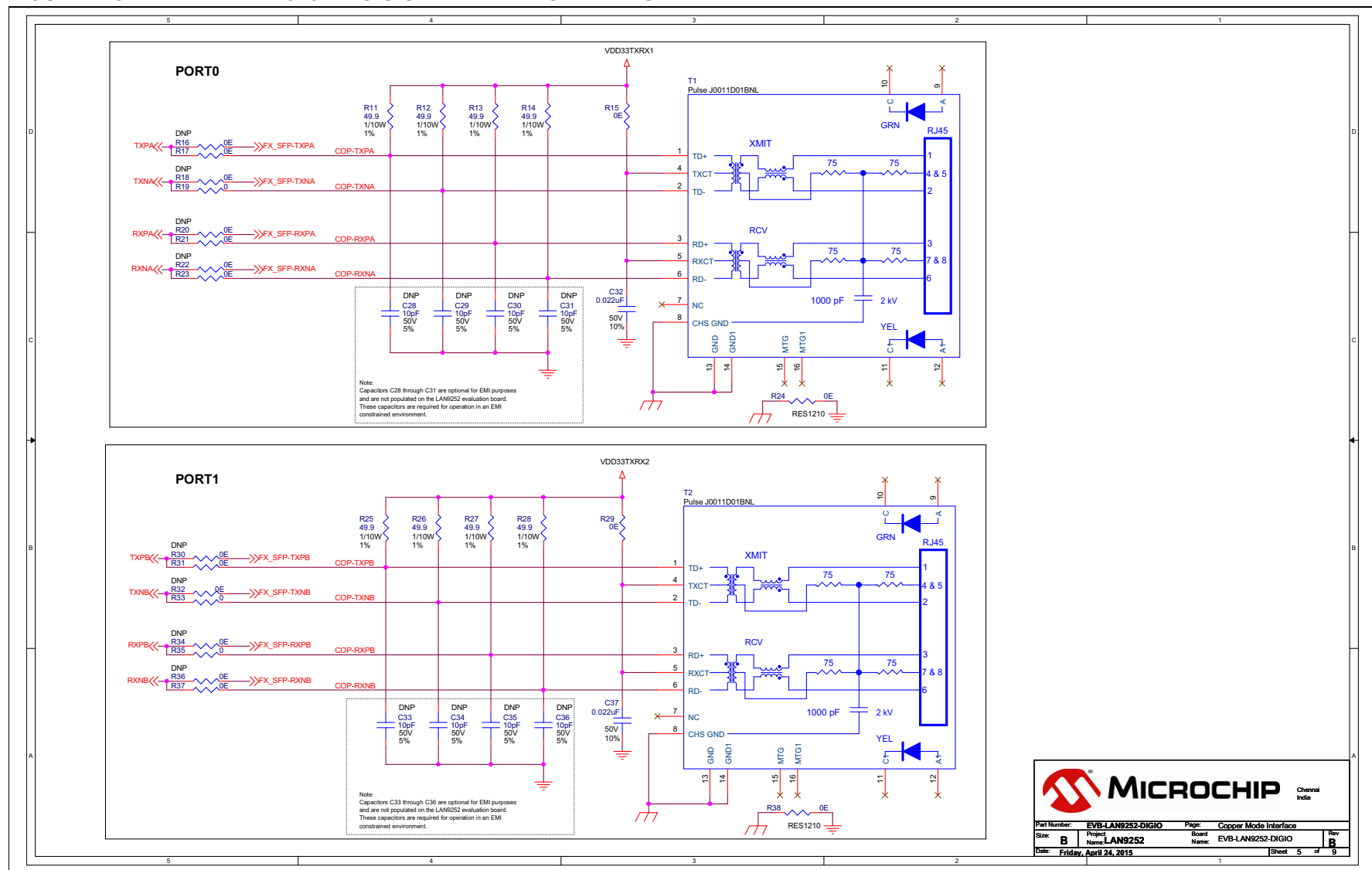
FIGURE B-3: EVB-LAN9252-DIGIO SCHEMATIC COPPER MODE INTERFACE
