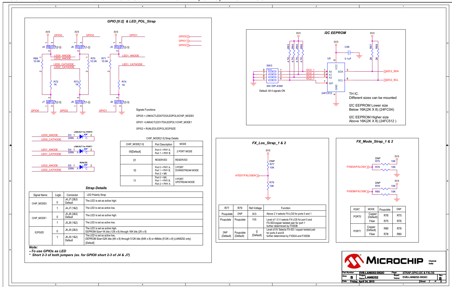
FIGURE B-5: EVB-LAN9252-DIGIO SCHEMATIC STRAP, GPIO, I2C &amp; FXLOS
