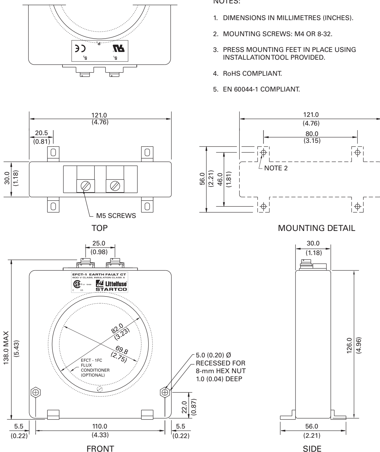
FIGURE 4. EFCT-1 Outline and Mounting Details.
