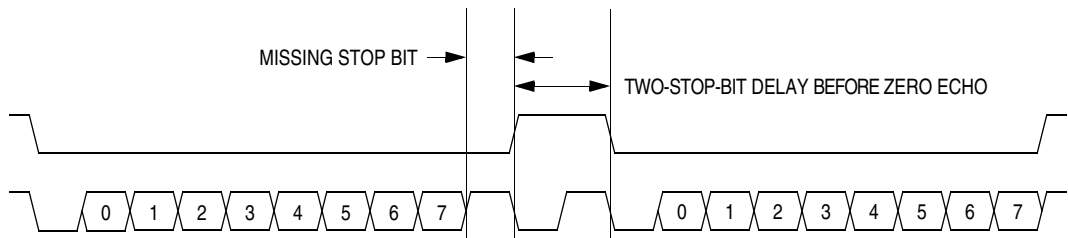
Figure 14-5. Break Transaction
