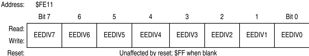
Figure 6-8. EEPROM-1 Divider Nonvolatile Register Low (EE1DIVLNVR)
