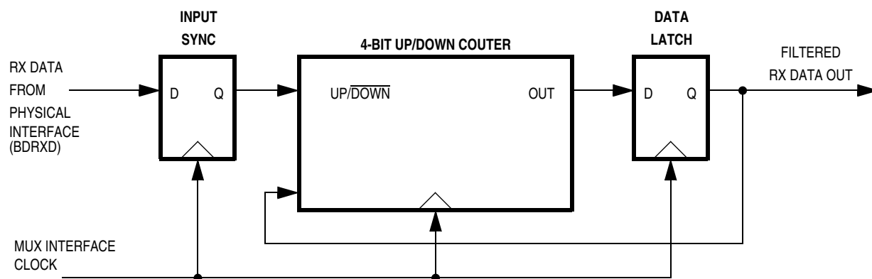
Figure 27-5. BDLC Rx Digital Filter Block Diagram
