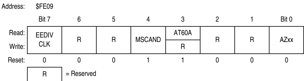
Figure 12-1. Configuration Register (CONFIG-2)
