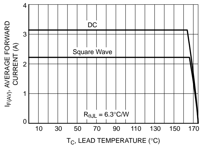
Figure 6. Current Derating
