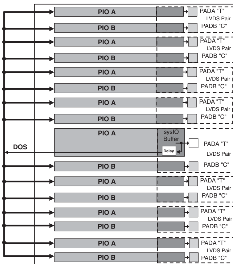
Figure 2-33. DQS Input Routing for the Left and Right Edges of the Device
