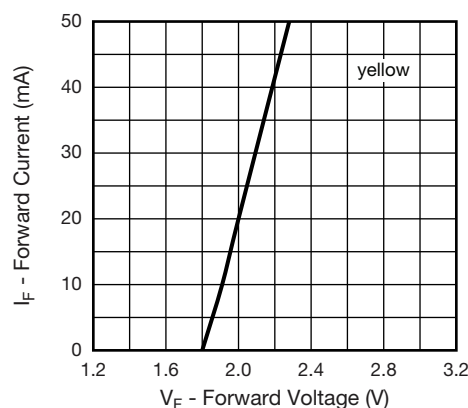
Fig. 4 - Forward Current vs. Forward Voltage (yellow)
