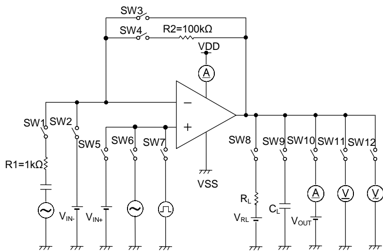
Figure 31. Test Circuit 2
