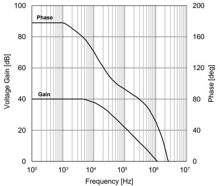
Figure 29. Voltage Gain · Phase vs Frequency ( V_{DD}=3.0\text{ V} )
