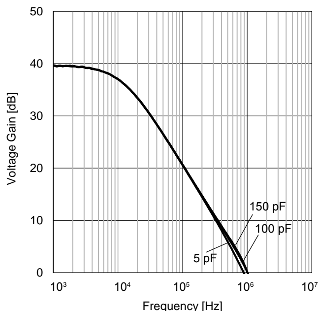
Figure 34. Voltage Gain vs Frequency ( V_{DD}=3.0 V, G_V=40 dB)
