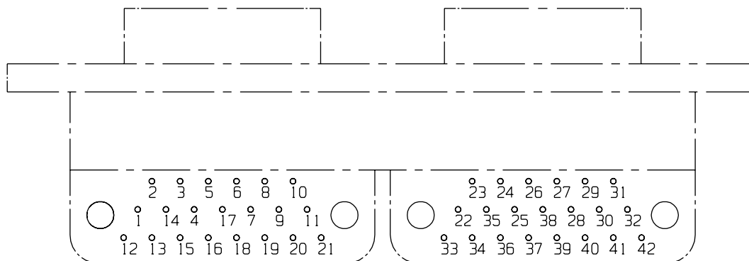
Termination Contact Identification
