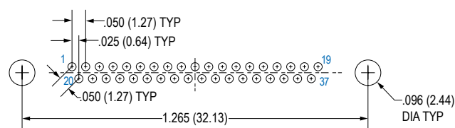
37 Contacts
