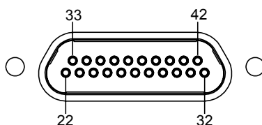
Mating Face Contact Identification
