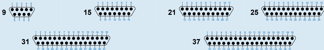
MICRO-D IN-LINE FILTER ADAPTER CONTACT ARRANGEMENTS
