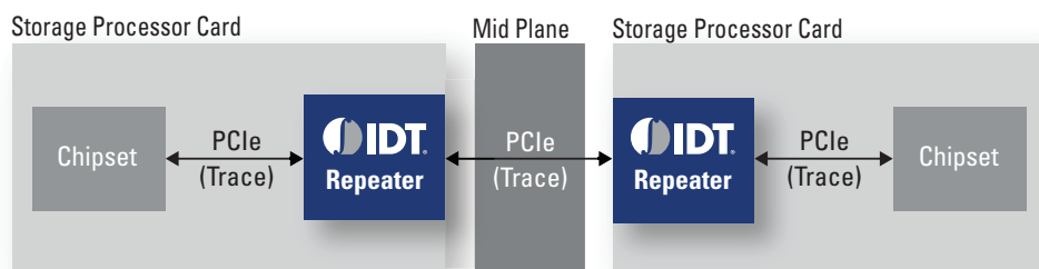
Figure 3: Storage Application
