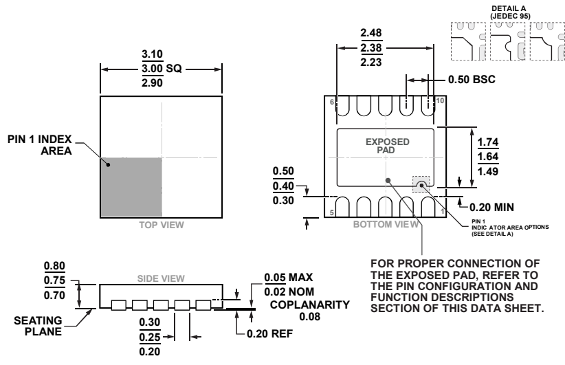
Figure 53. 10-Lead Lead Frame Chip Scale Package [LFCSPP] 3 mm × 3 mm Body and 0.75 mm Package Height (CP-10-9)
