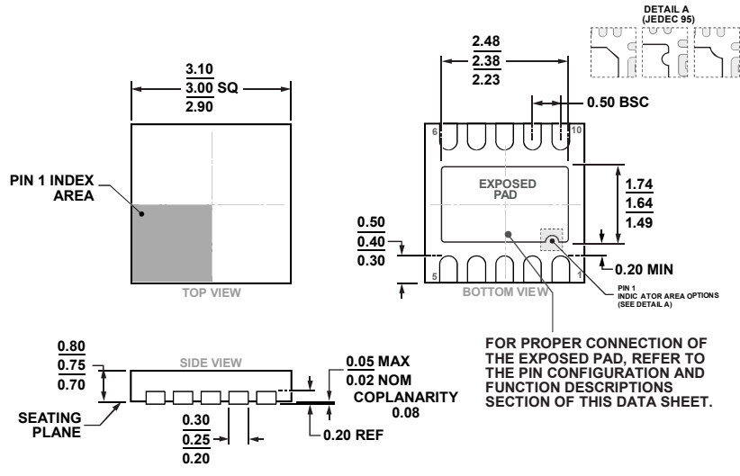
Figure 53. 10-Lead Lead Frame Chip Scale Package [LFCS] 3 mm × 3 mm Body and 0.75 mm Package Height (CP-10-9) Dimensions shown in millimeters
