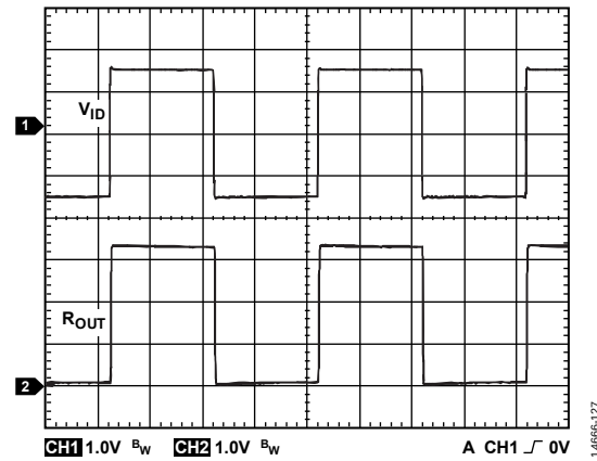
Figure 24. Receiver Propagation Delay (Oscilloscope Plot), Data Rate = 500 kbps, V_{DD} \geq 1.5 V
