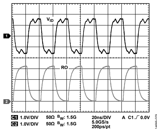
Figure 32. Receiver Propagation Delay (Oscilloscope Plot) at 50 Mbps, |V_{IO}| \geq 1.5 V
