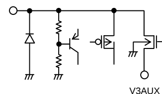
17pin&lt;V3AUX_IN&gt;
