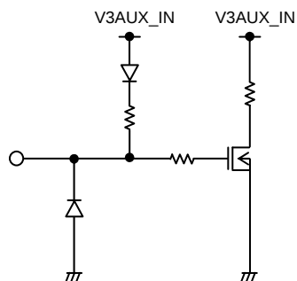
20pin&lt;EN&gt;
