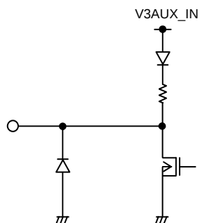
18pin&lt;RCLKEN &gt;
