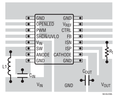
Figure 5. Suggested Layout
