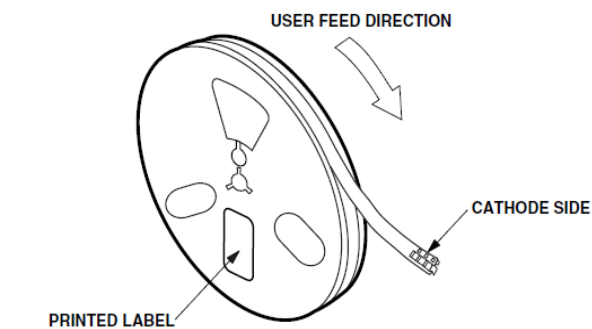
Figure 12: Reel Orientation
