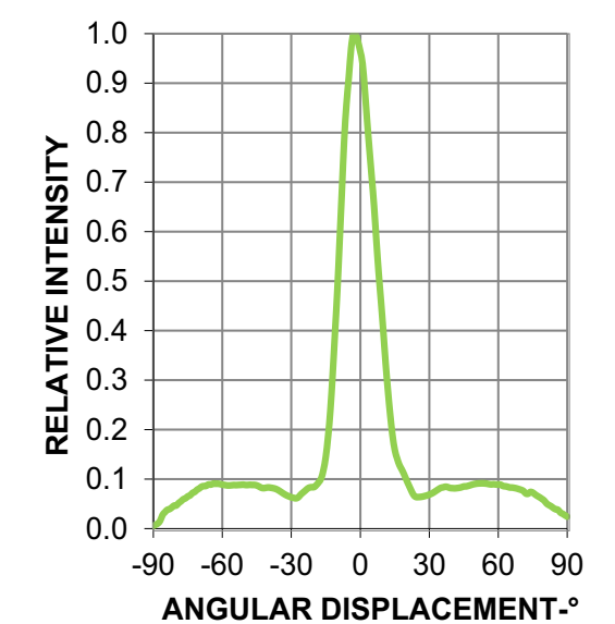
Figure 5: Radiation Pattern
