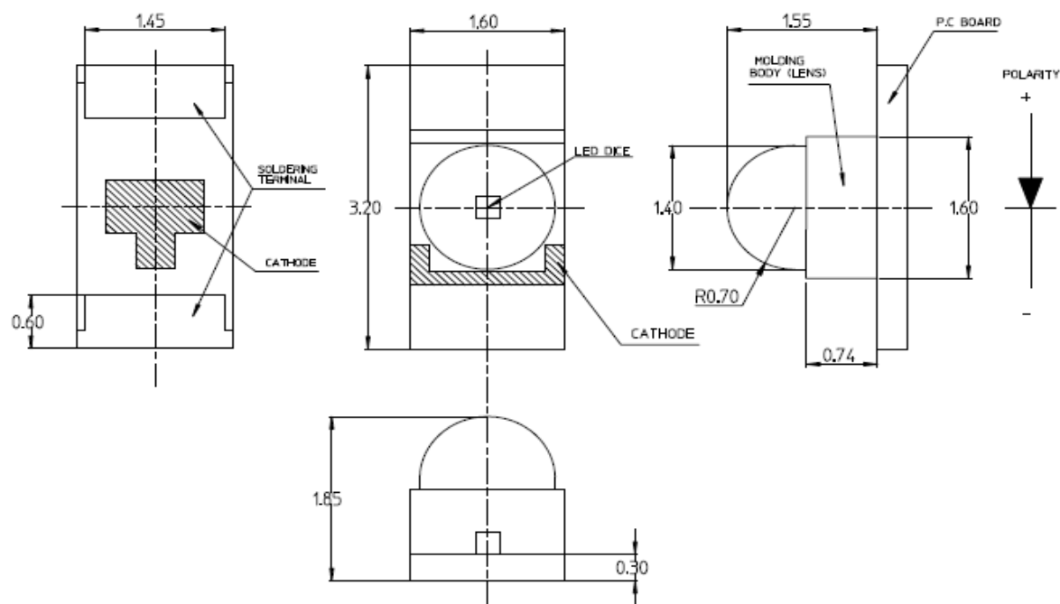
Figure 1: Package Dimensions
