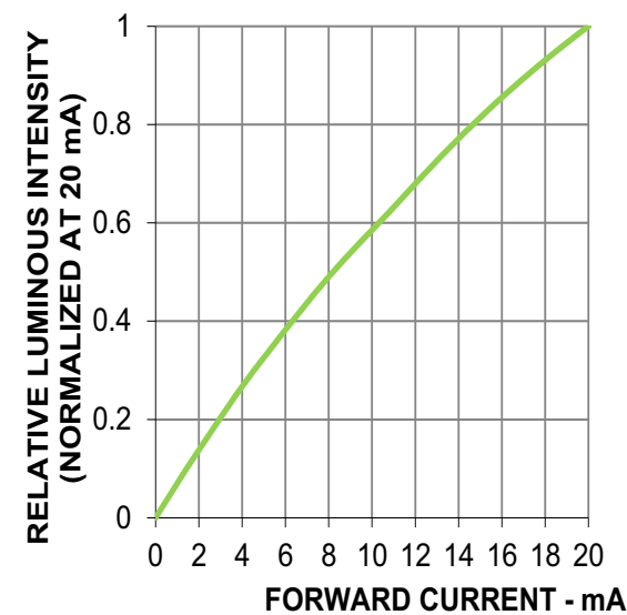
Figure 3: Luminous Intensity vs. Forward Current
