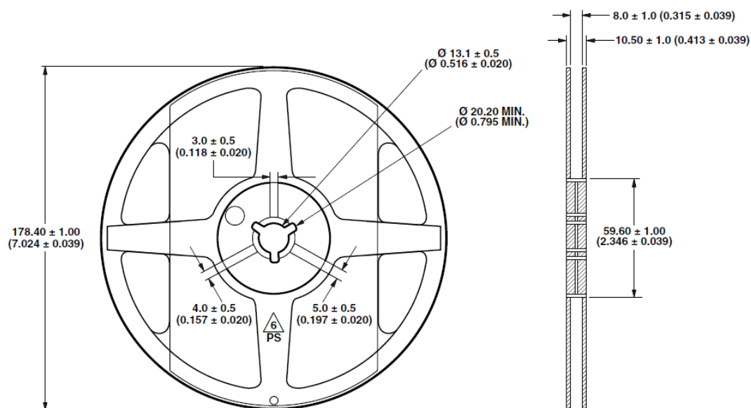
Figure 13: Reel Dimensions
