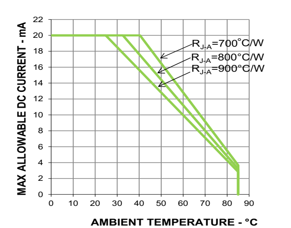
Figure 10: Derating Curve
