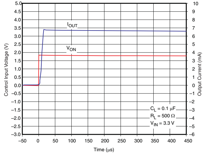
Figure 21. t_{ON} Response
