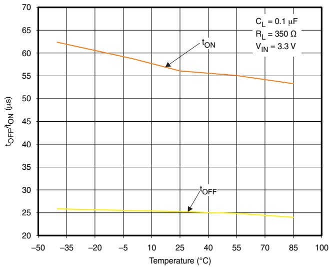
Figure 16. t_{ON}/t_{OFF}
