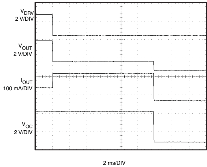
Figure 19. t_{BLANK} Response
