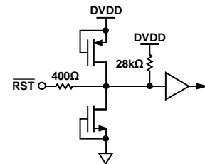
Figure 27. Equivalent RST Input Circuit
