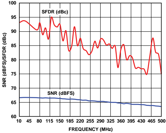
Figure 11. Single-Tone SNR/SFDR vs. Input Frequency ( f_{IN} )
