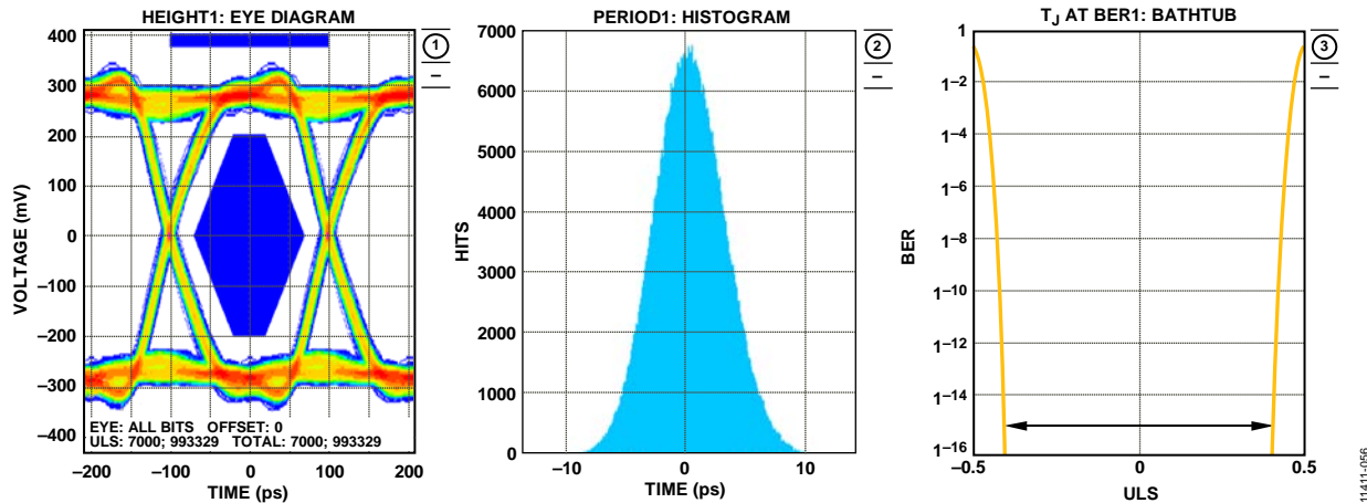
Figure 56. AD6677 Digital Outputs Data Eye, Histogram, and Bathtub, External 100 Ω Terminations at 5 Gbps
