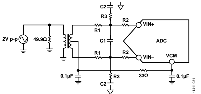
Figure 31. Differential Transformer-Coupled Configuration
