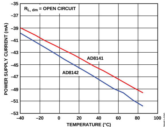
Figure 29. Negative Power Supply Current vs. Temperature
