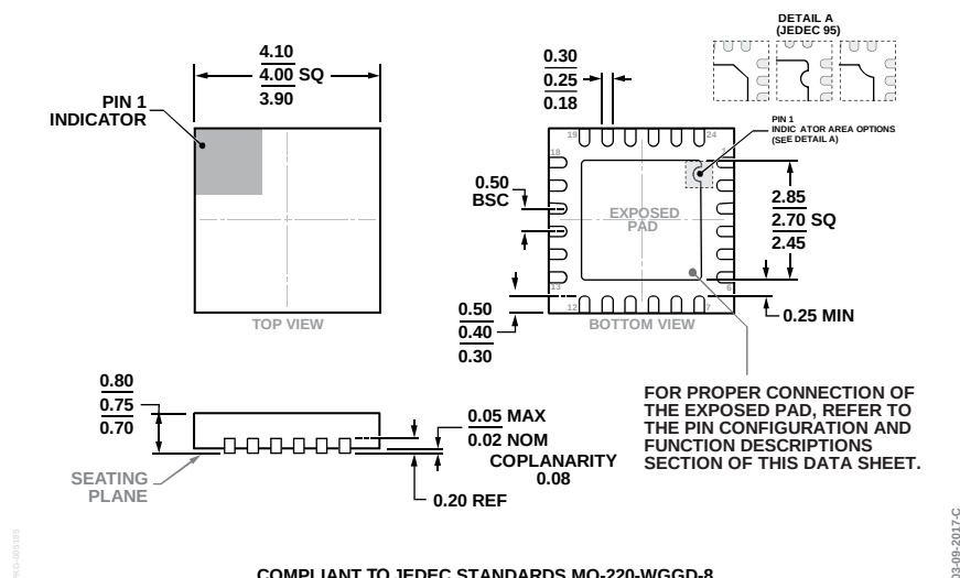
Figure 50. 24-Lead Lead Frame Chip Scale Package [LFCSP] 4 mm × 4 mm Body and 0.75 mm Package Height (CP-24-8) Dimensions shown in millimeters
