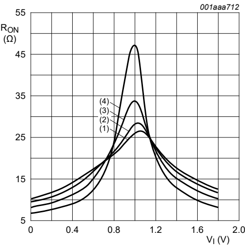
V_{CC} = 1.8\text{ V} 1. T_{amb} = 125^\circ\text{C} 2. T_{amb} = 85^\circ\text{C} 3. T_{amb} = 25^\circ\text{C} 4. T_{amb} = -40^\circ\text{C}
