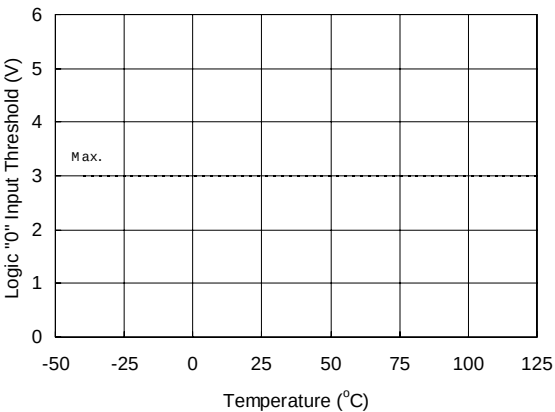
Figure 13A. Logic "0" Input Threshold vs. Temperature
