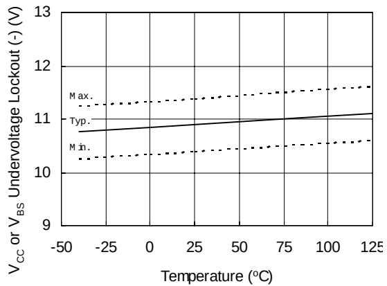
Figure 19. V_{CC} or V_{BS} Undervoltage (-) vs. Temperature
