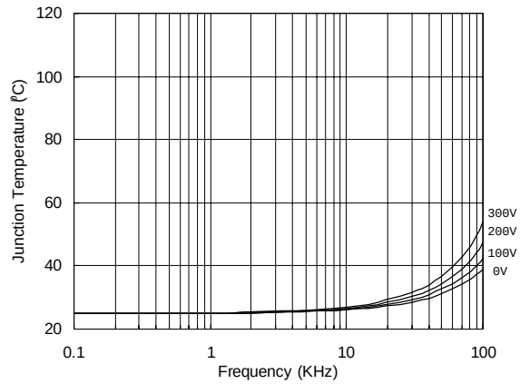
Figure 41. IR21363 (J) vs. Frequency (IRG4PC50W), R_{gate}=5\Omega , V_{cc}=15V
