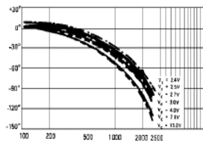
Phase vs. V_{\text{CONTROL}} vs. Frequency
