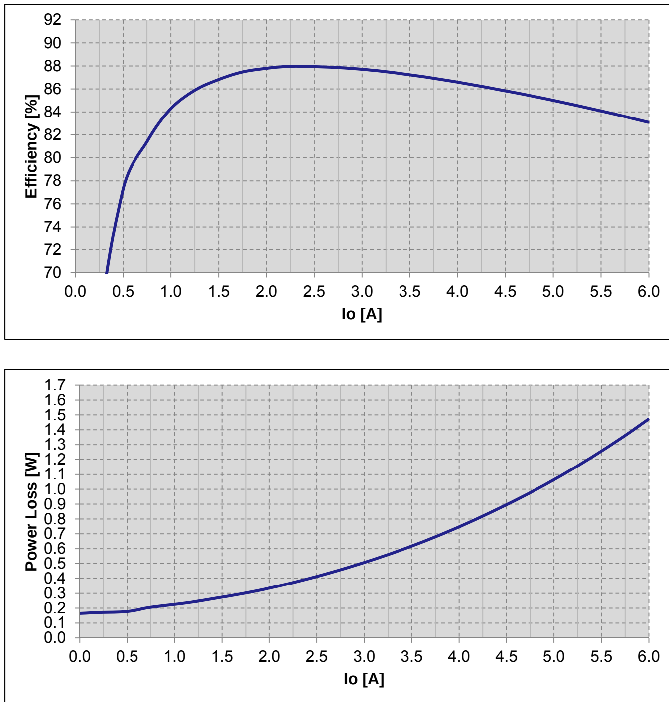
Fig.20: Efficiency and power loss vs. load current for channel2 ( V_{out2} = 1.2V )
