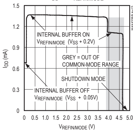
I_{DD} vs. V_{REFIN/MODE}
