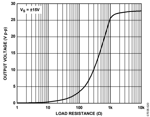
Figure 26. Output Voltage Swing vs. Load Resistance
