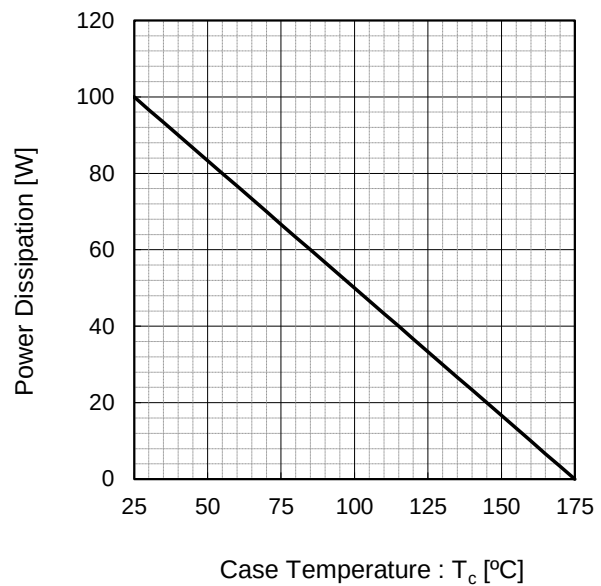
Fig.6 Power Dissipation
