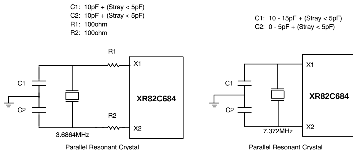
Figure 29. Recommended Schematics for the XTAL Oscillator Circuitry
