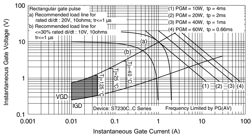
Fig. 11 - Gate Characteristics
