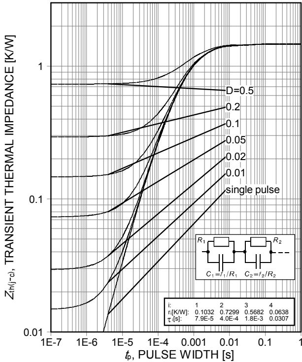
Figure 21. IGBT transient thermal impedance as a function of pulse width 1) (see page 4) ( D = \phi_p/T )
