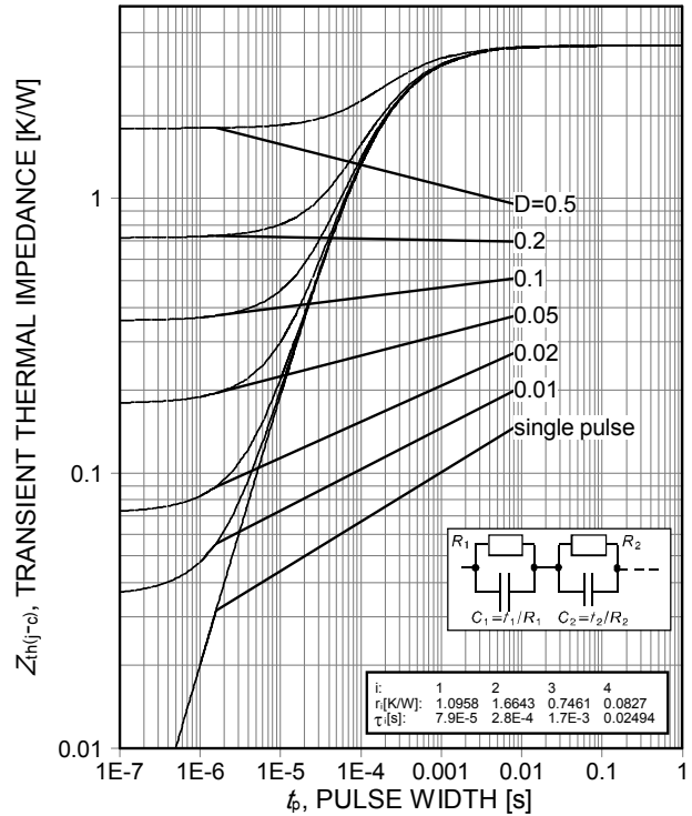
Figure 22. Diode transient thermal impedance as a function of pulse width 2) (see page 4) ( D = \phi_p/T )
