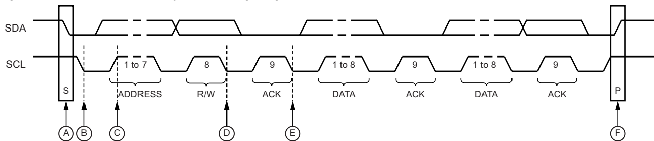
Figure 4-66. Two-wire Mode, Typical Timing Diagram
