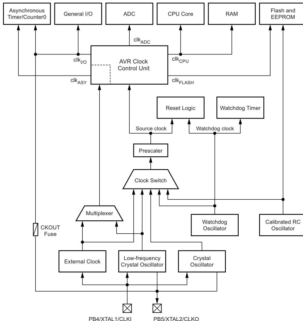
Figure 4-10. Clock Distribution
