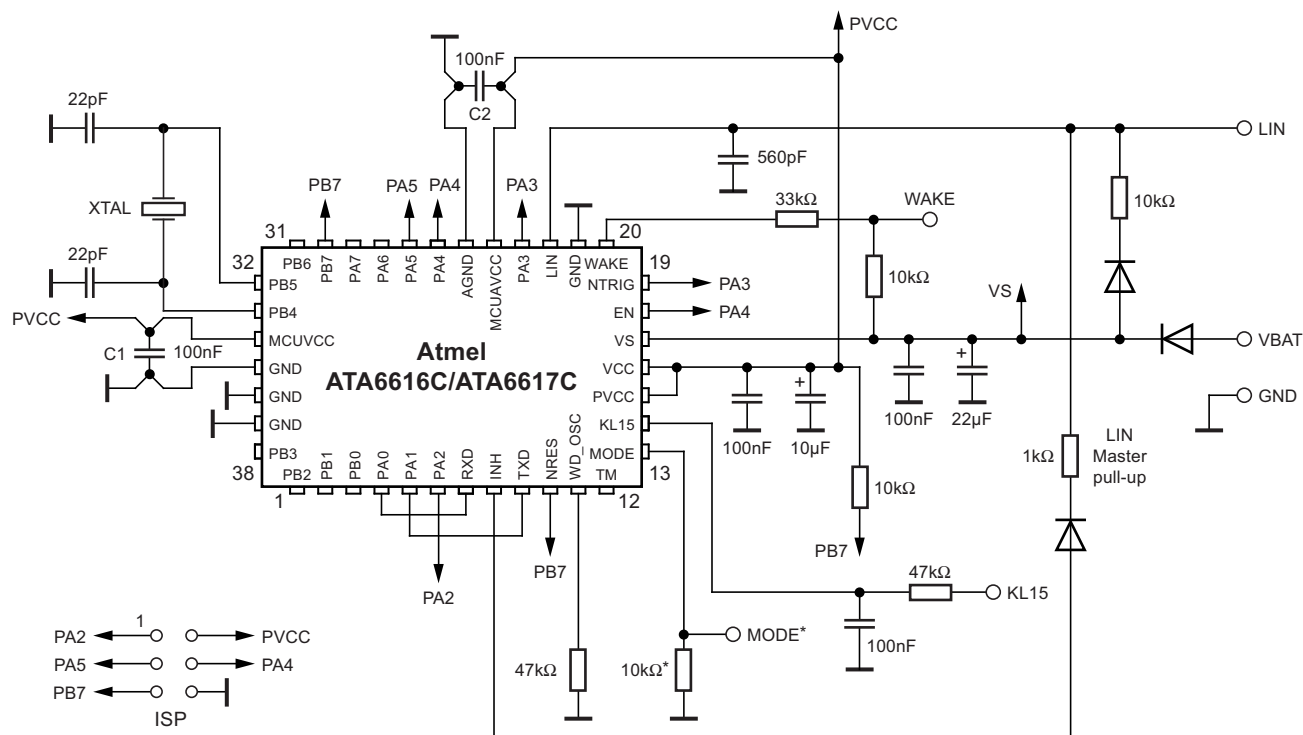
Figure 5-3. Typical LIN Master Application 1kΩ LIN Master Pull-up Switched Off during Sleep and Silent Mode
