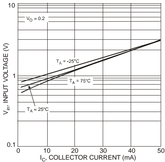
Fig. 28 Input Voltage vs. Collector Current
