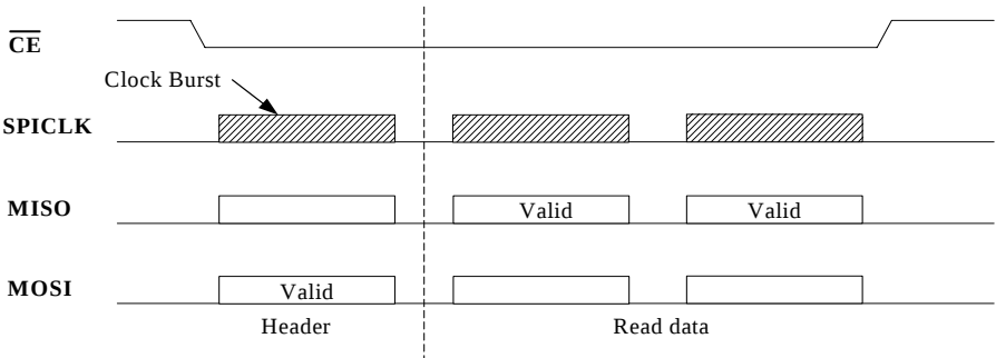
Figure 9. SPI Read Transaction Diagram
