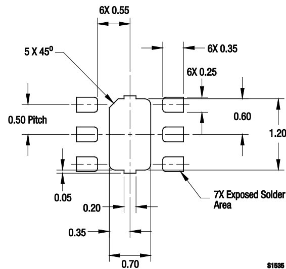
Figure 12. SKY13438-374LF PCB Layout Footprint (Top View)
