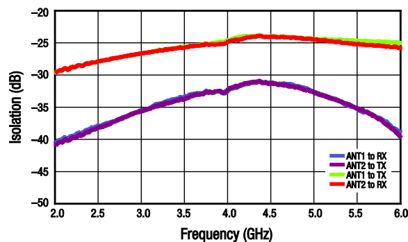
Figure 4. Isolation vs Frequency (ANT1 or ANT2 to TX or RX)
